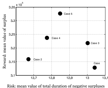
Fig. 11. The efficient frontier under Gaussian copula with catastrophe event
